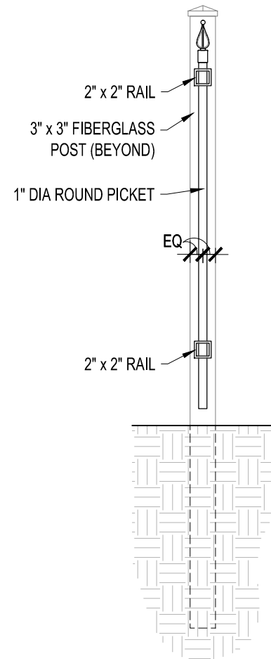
02 FENCE SECTION
