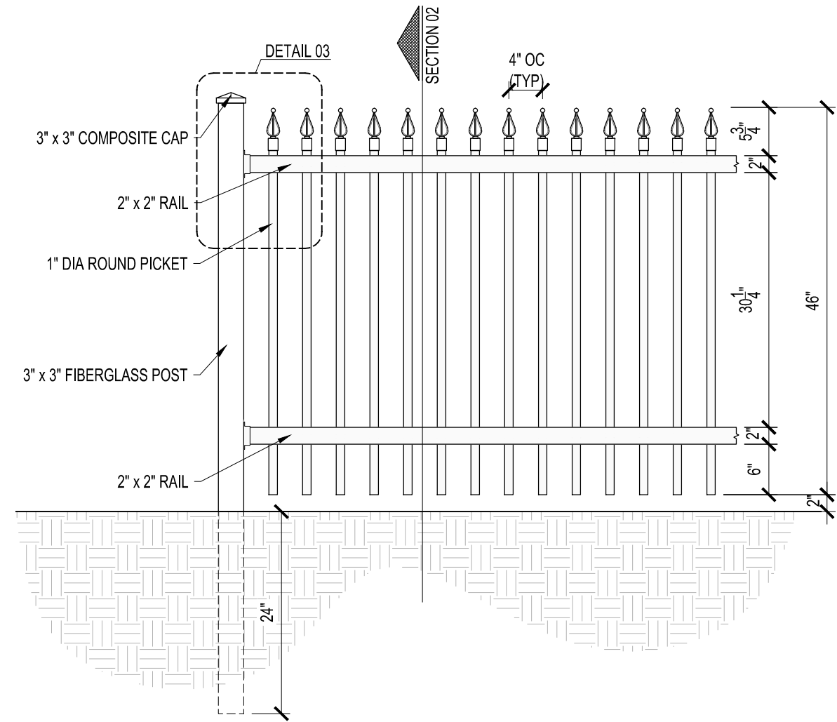
01 FENCE ELEVATION
